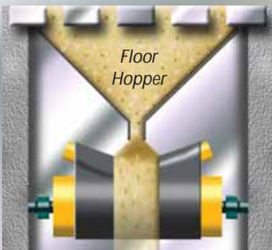
The V-positioned support rollers help to secure a controlled abrasive load, save energy and avoid spillage
