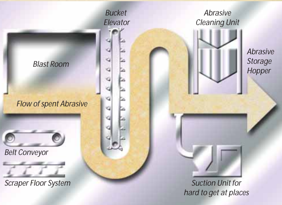
The Munkebo Recovery System for fixed installations
